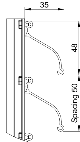
DETAIL C SCALE 1 : 2
